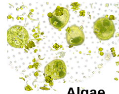
Algae Phytoplankton
